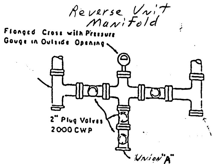
PLAN VIEW - MANIFOLD
