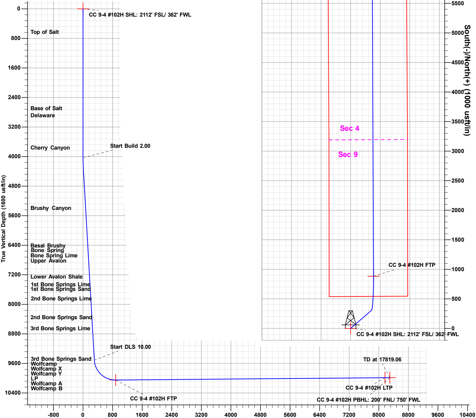
Vertical Section at 359.77° (1600 usft/in)
