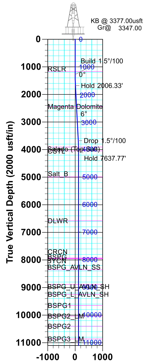
Vertical Section at 180.05° (2000 usft/in)
