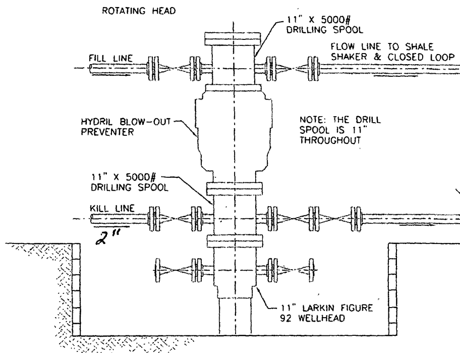
WELLHEAD ELEVATION
