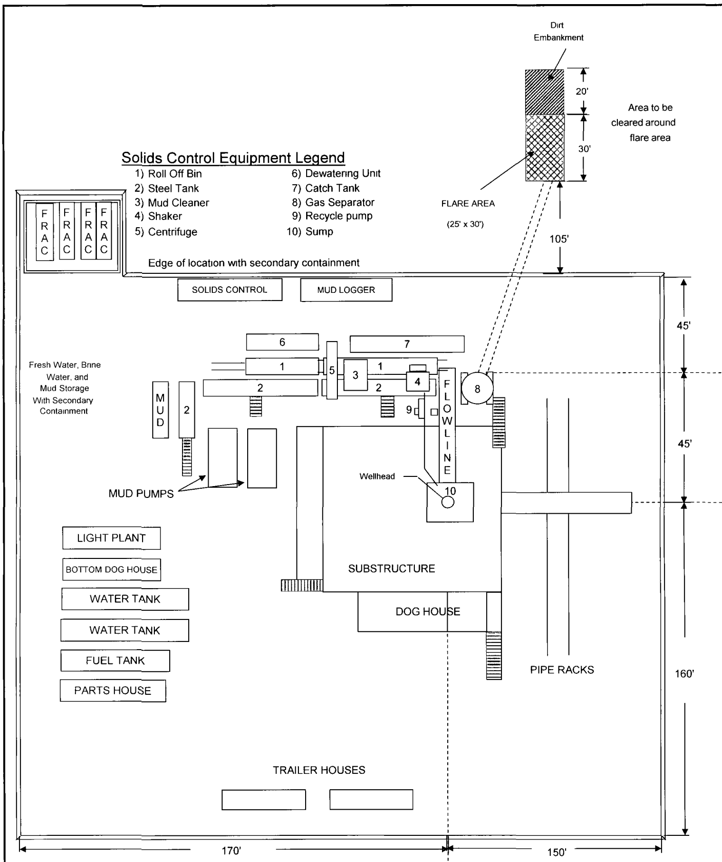
POKER LAKE UNIT 392H TYPICAL RIG LAYOUT SCHEMATIC INCLUSIVE OF CLOSED-LOOP DESIGN PLAN
