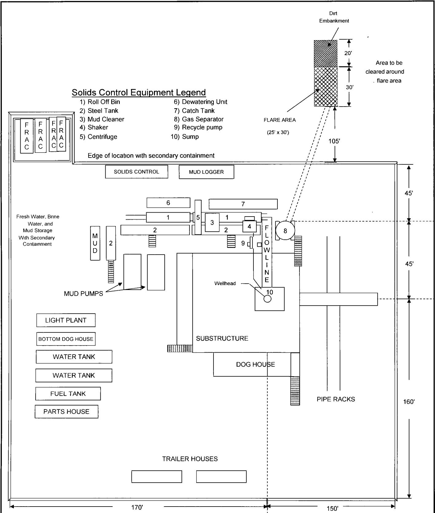
POKER LAKE UNIT 364H TYPICAL RIG LAYOUT SCHEMATIC INCLUSIVE OF CLOSED-LOOP DESIGN PLAN
