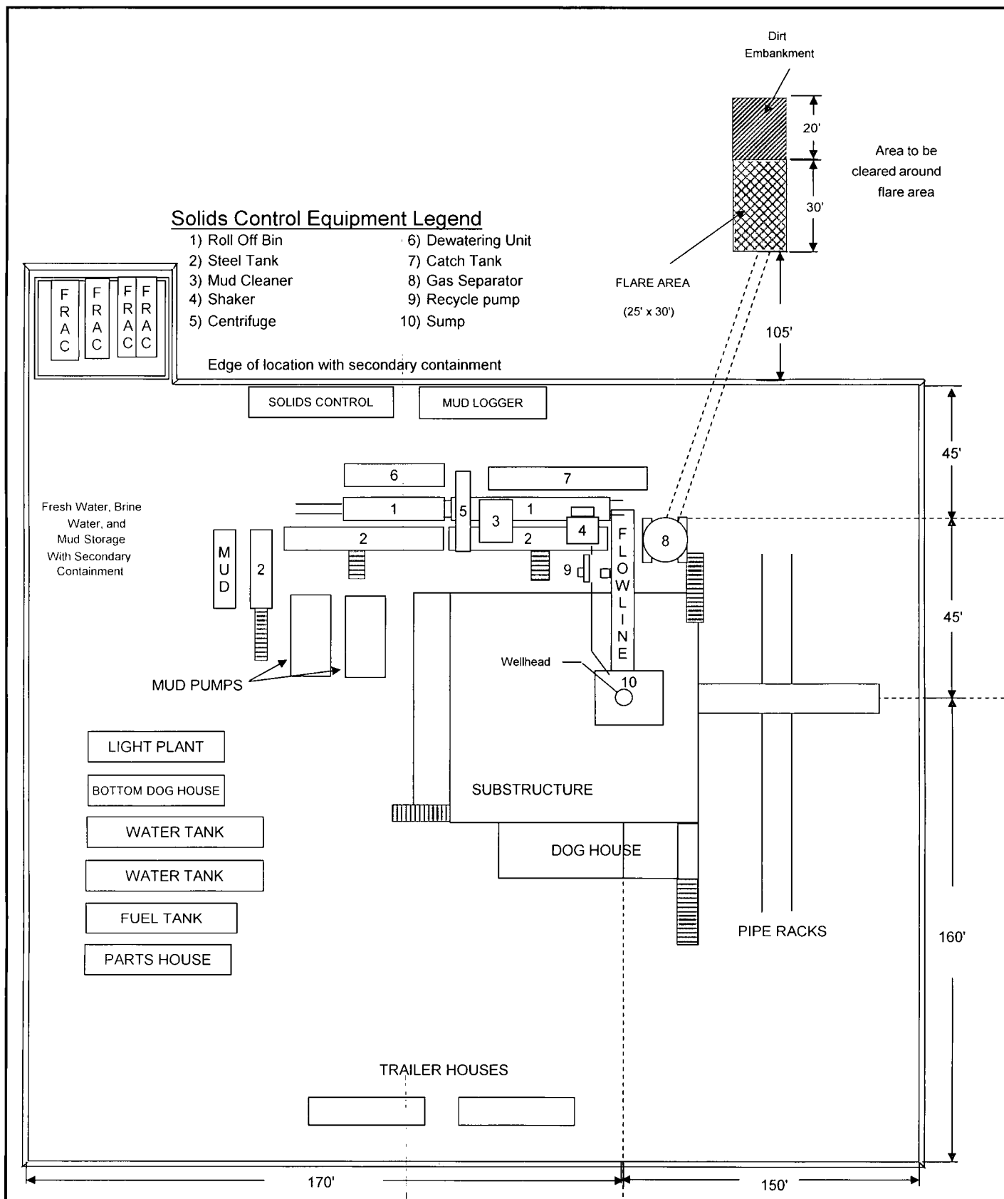
POKER LAKE UNIT 443H TYPICAL RIG LAYOUT SCHEMATIC INCLUSIVE OF CLOSED-LOOP DESIGN PLAN
