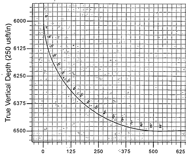
Vertical Section at 88.04° (250 usft/in)
