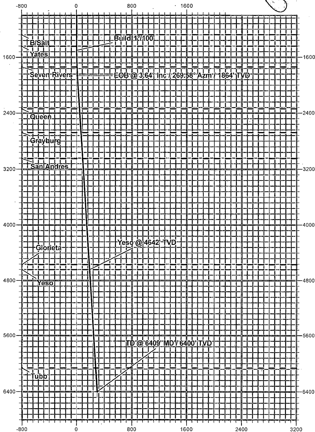
Vertical Section at 269.58° (800 usft/in)
