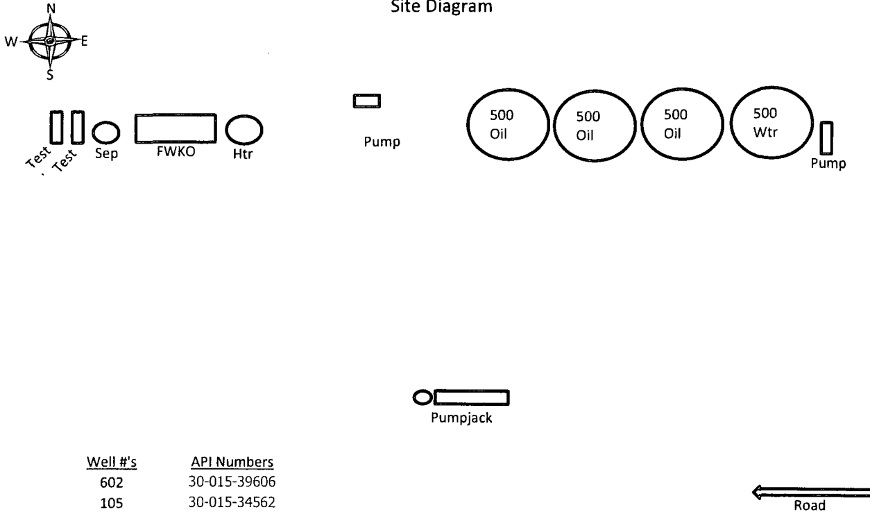
Site Diagram
