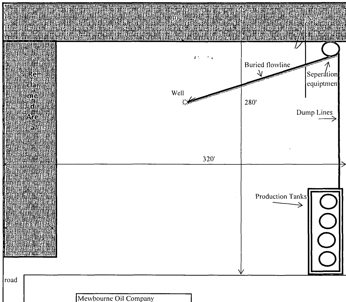
Closed Loop Pad Dimensions 280' x 320'
