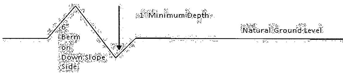
Cross Section of a Typical Lead-off Ditch
