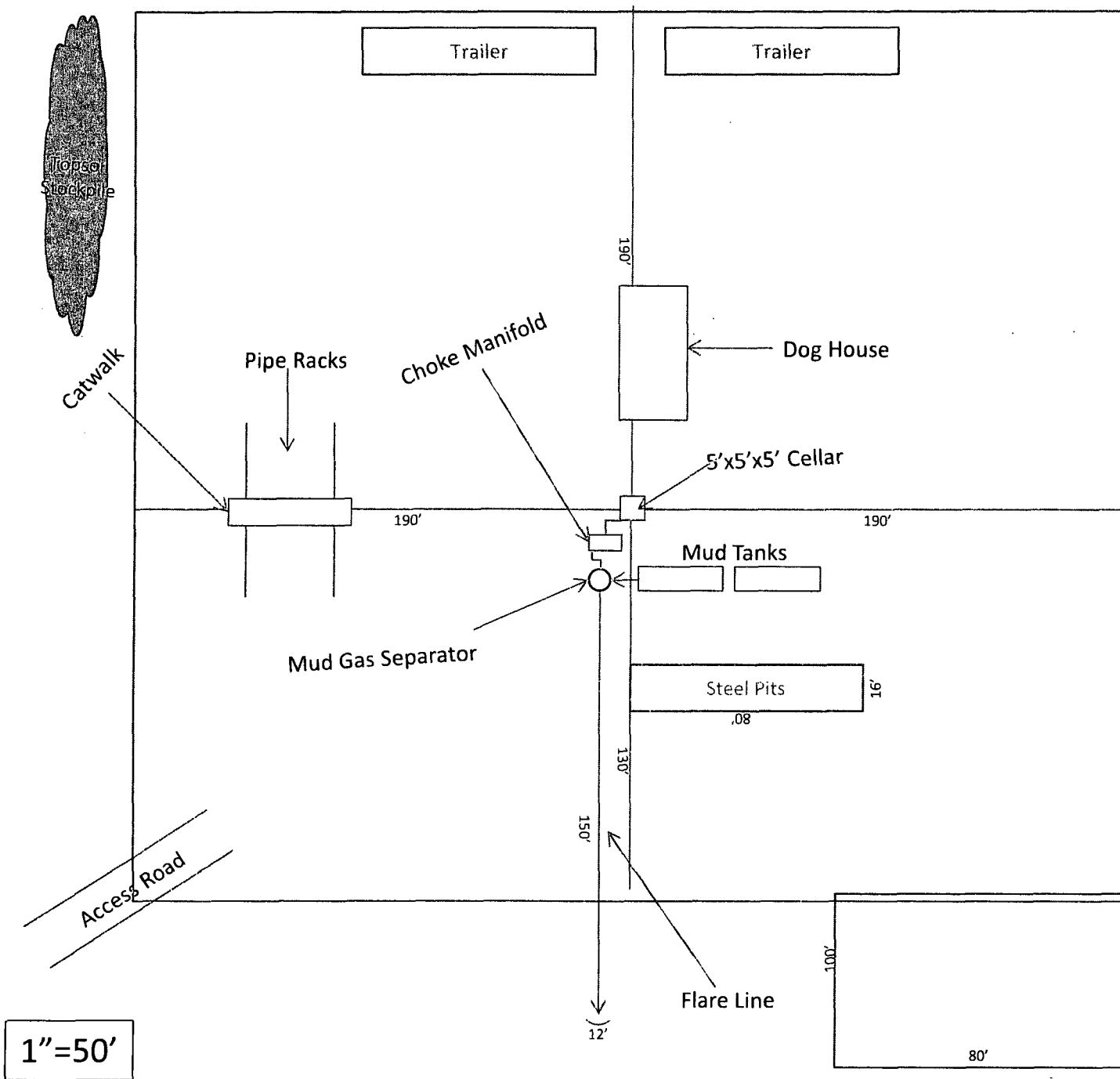
Exhibit D – Rig Diagram Parks Federal Com No. 2 Cimarex Energy Co. of Colorado 9-25S-26E SHL 990 FSL & 330 FEL BHL 850 FSL & 330 FWL Eddy County, NM
