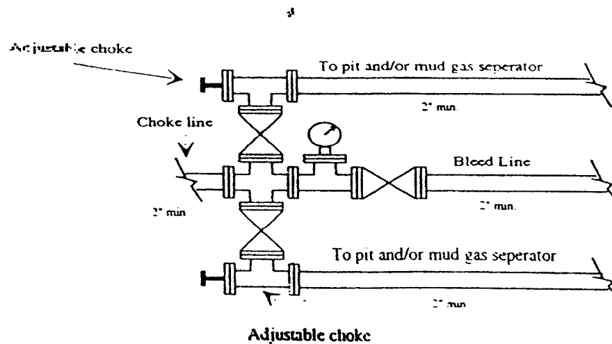
Typical 2,000 psi choke manifold assembly with at least these minimum features
