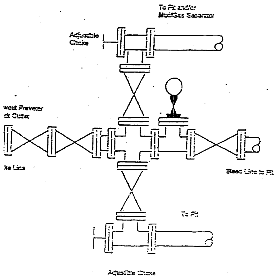
Choke Manifold Assembly for 3M WP System
