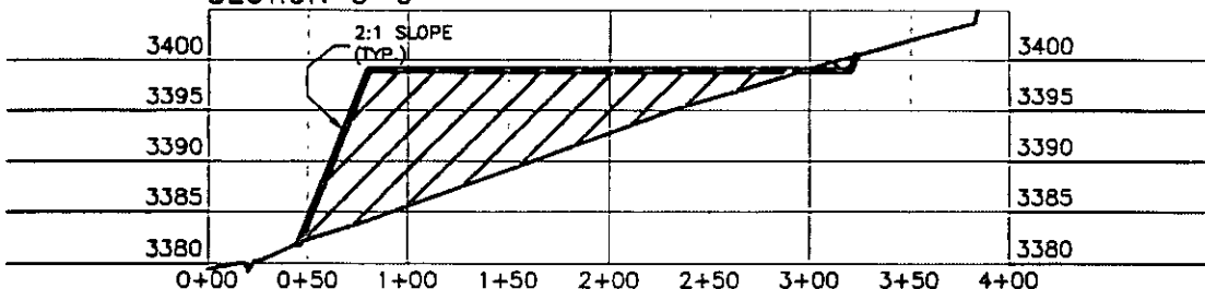
SECTION C-C'
