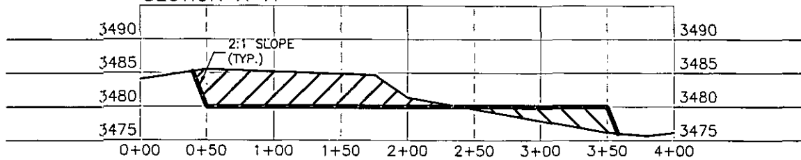
SECTION B-B'
