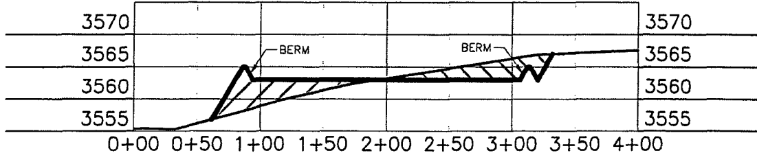
SECTION C-C'
