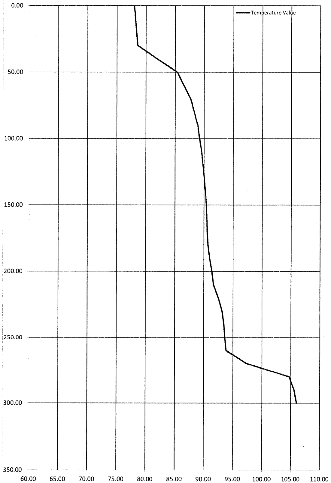
Stebbins 20 Fed #134H Temp Log
