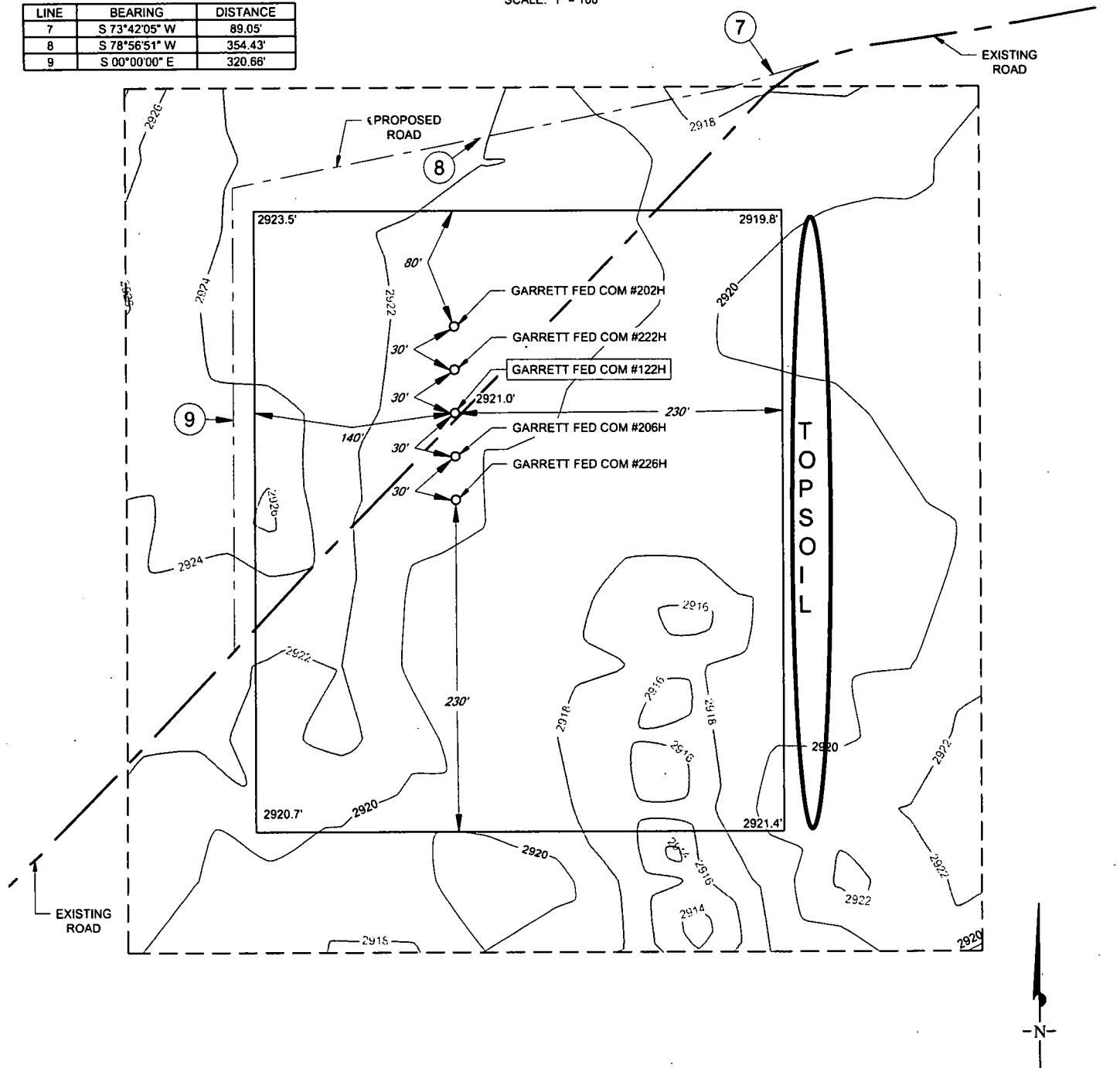
PROPOSED ROAD LINE TABLE
