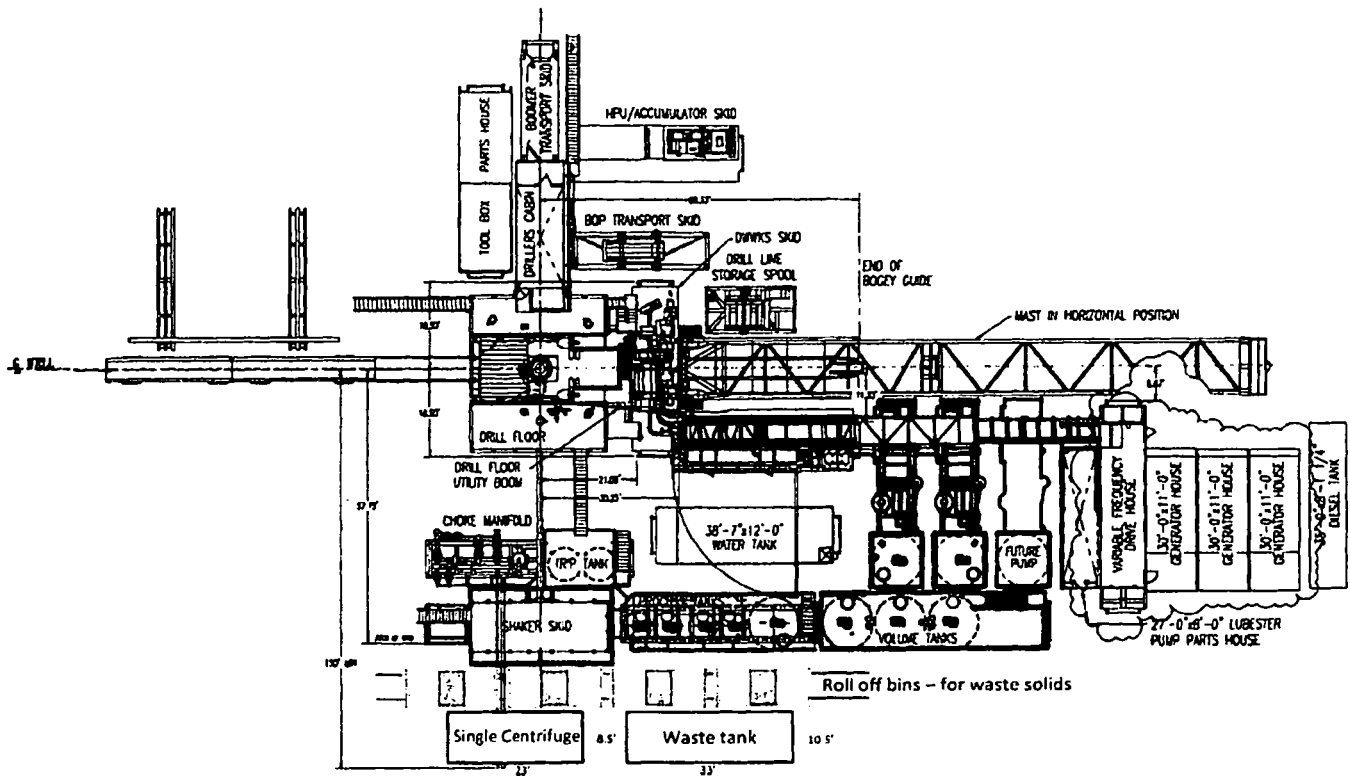
Rig Layout Diagram
