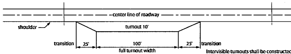
Typical Turnout Plan
