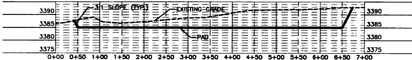
SECTION C-C'
