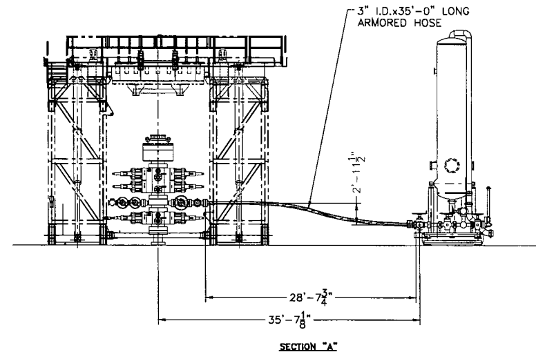
SECTION "A"
