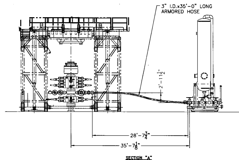
SECTION "A"
