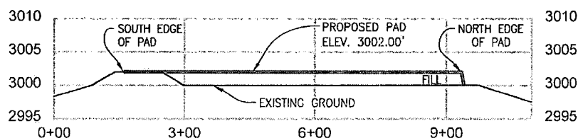
SECTION B-B
