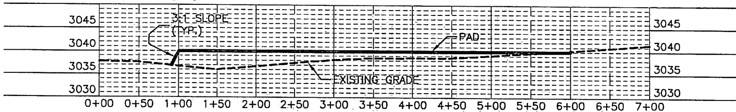
SECTION C-C'
