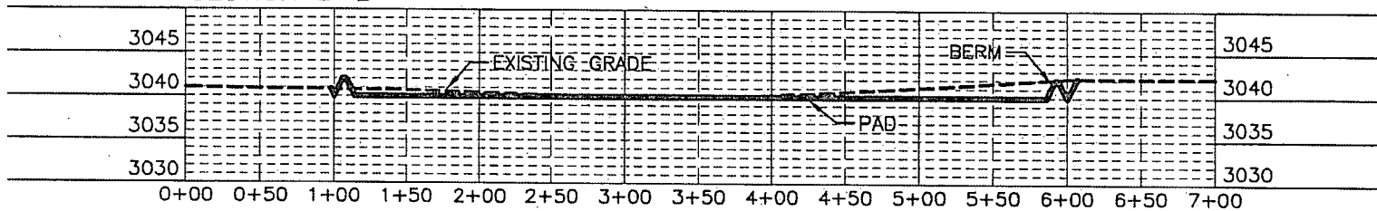
SECTION B-B'
