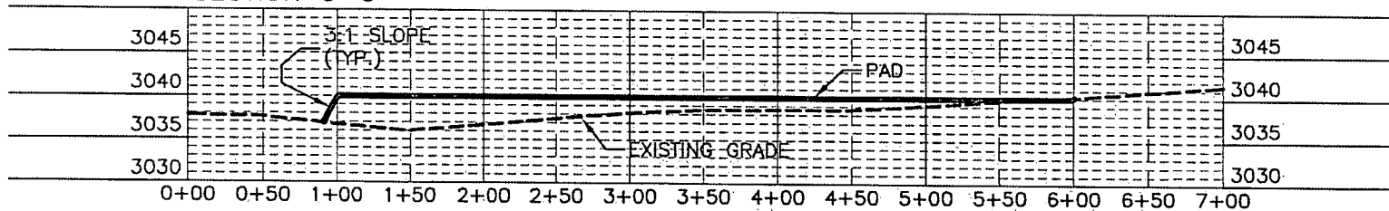
SECTION C-C'
