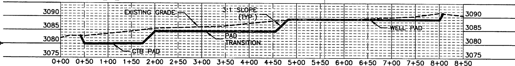
SECTION E-E'
