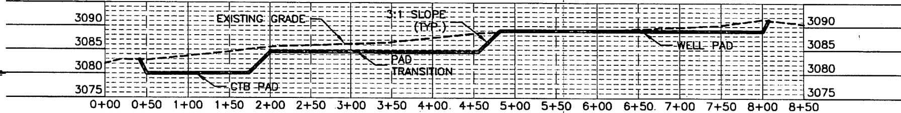
SECTION E-E'
