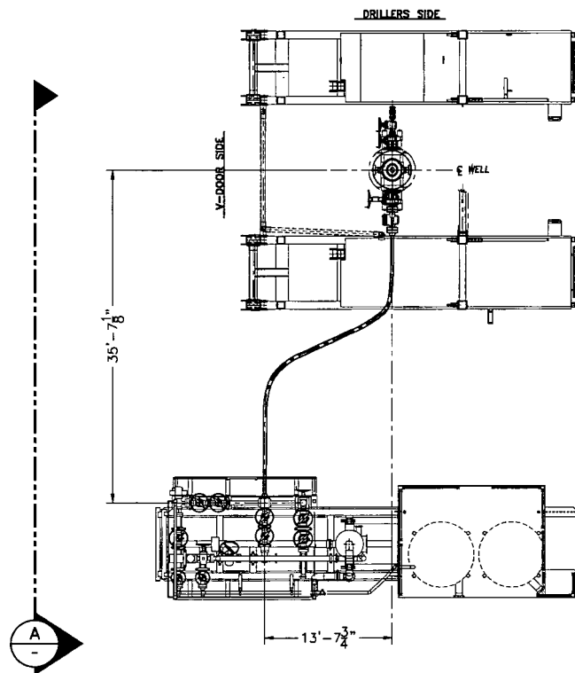
PLAN VIEW
