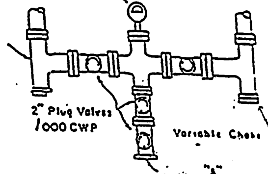
PLAN VIEW - CHOKES MANIFOLD
