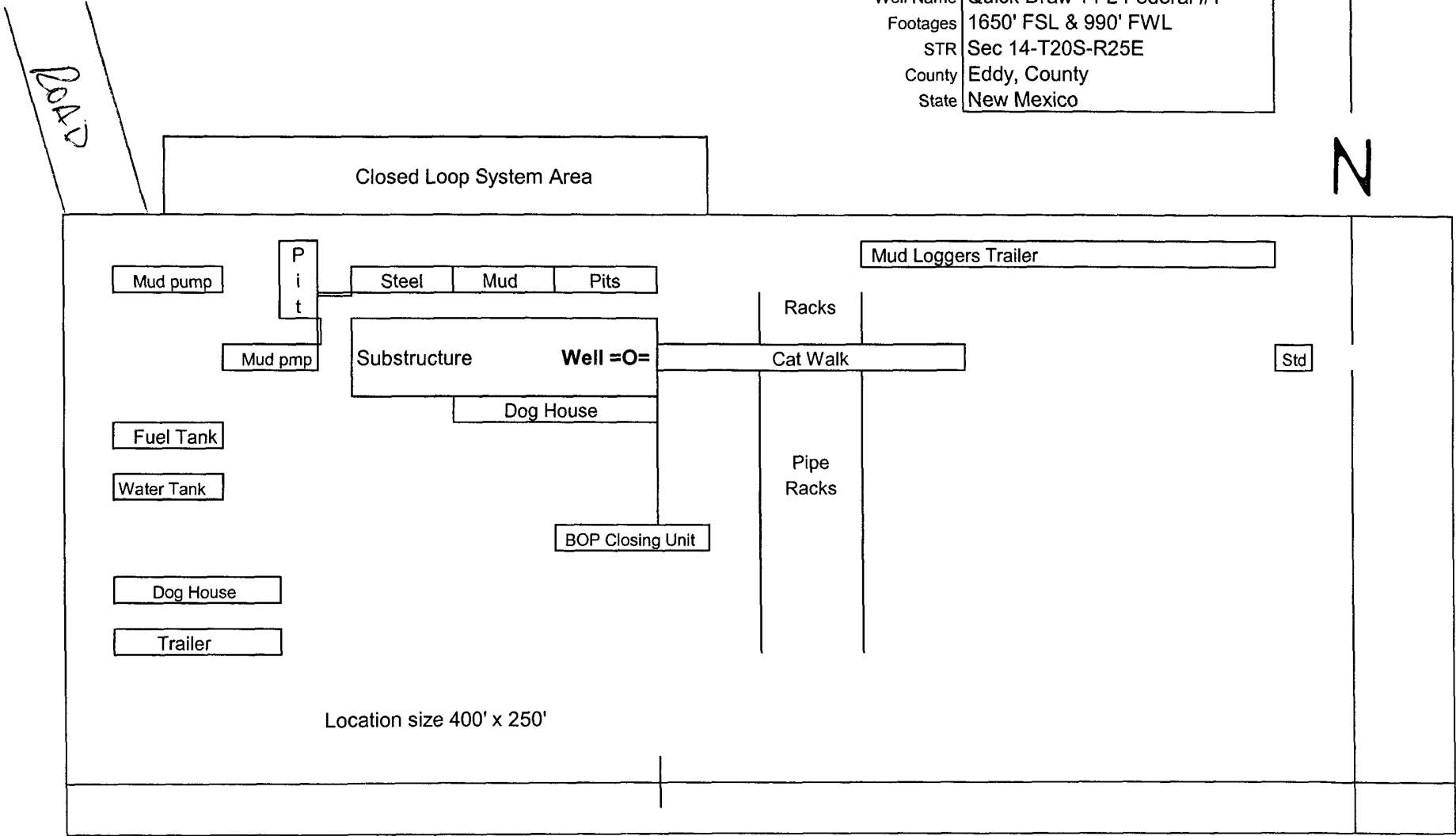
Rig Location Schematic
