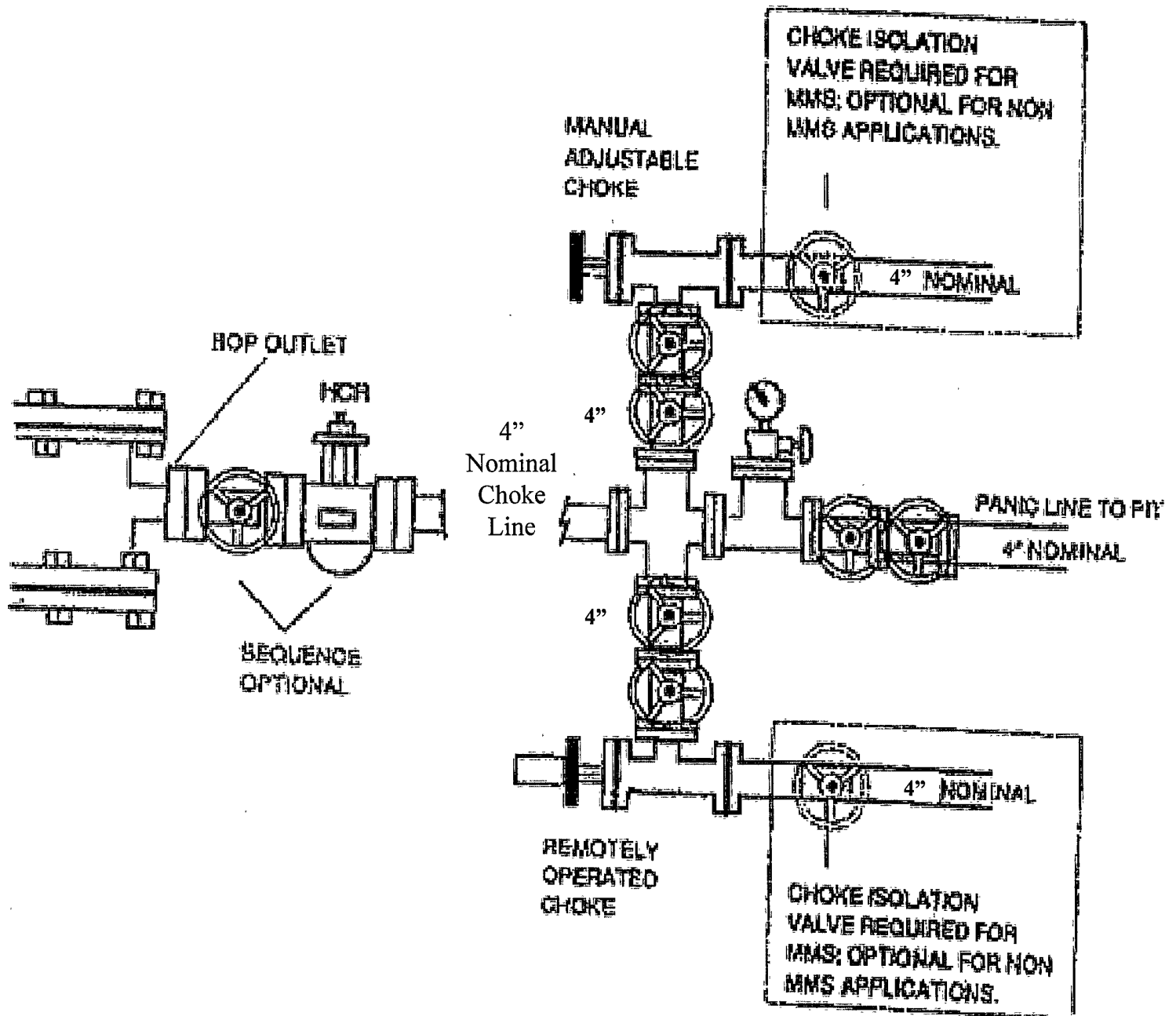
Exhibit E-1 – Choke Manifold Diagram Goldeneye 26 Federal No. 3 Cimarex Energy Co. of Colorado 26-25S-26E SHL 330 FSL & 600 FWL BHL 2310 FSL & 600 FWL Eddy County, NM
