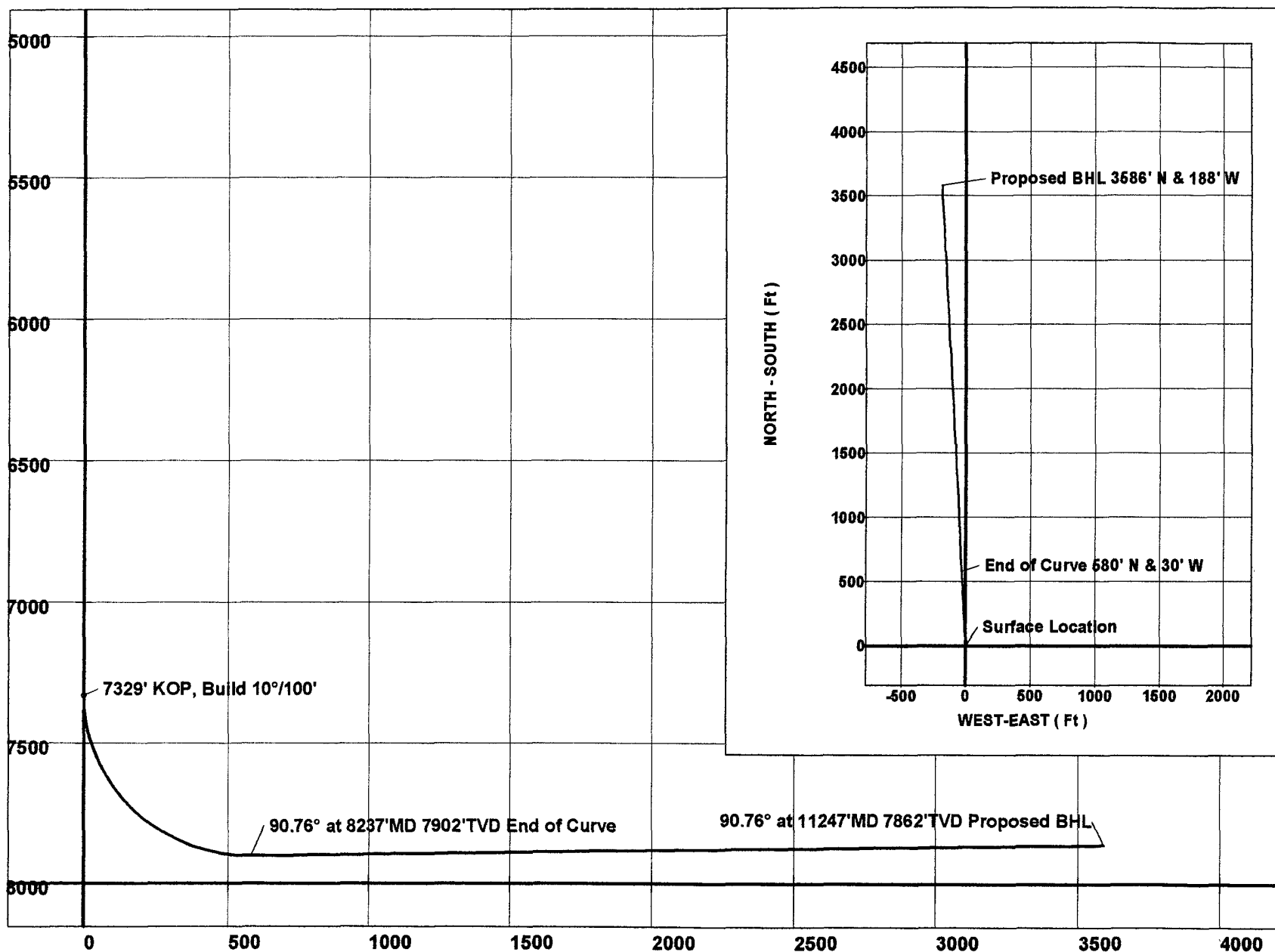
VERTICAL SECTION ( Ft ) @ 357.00°
