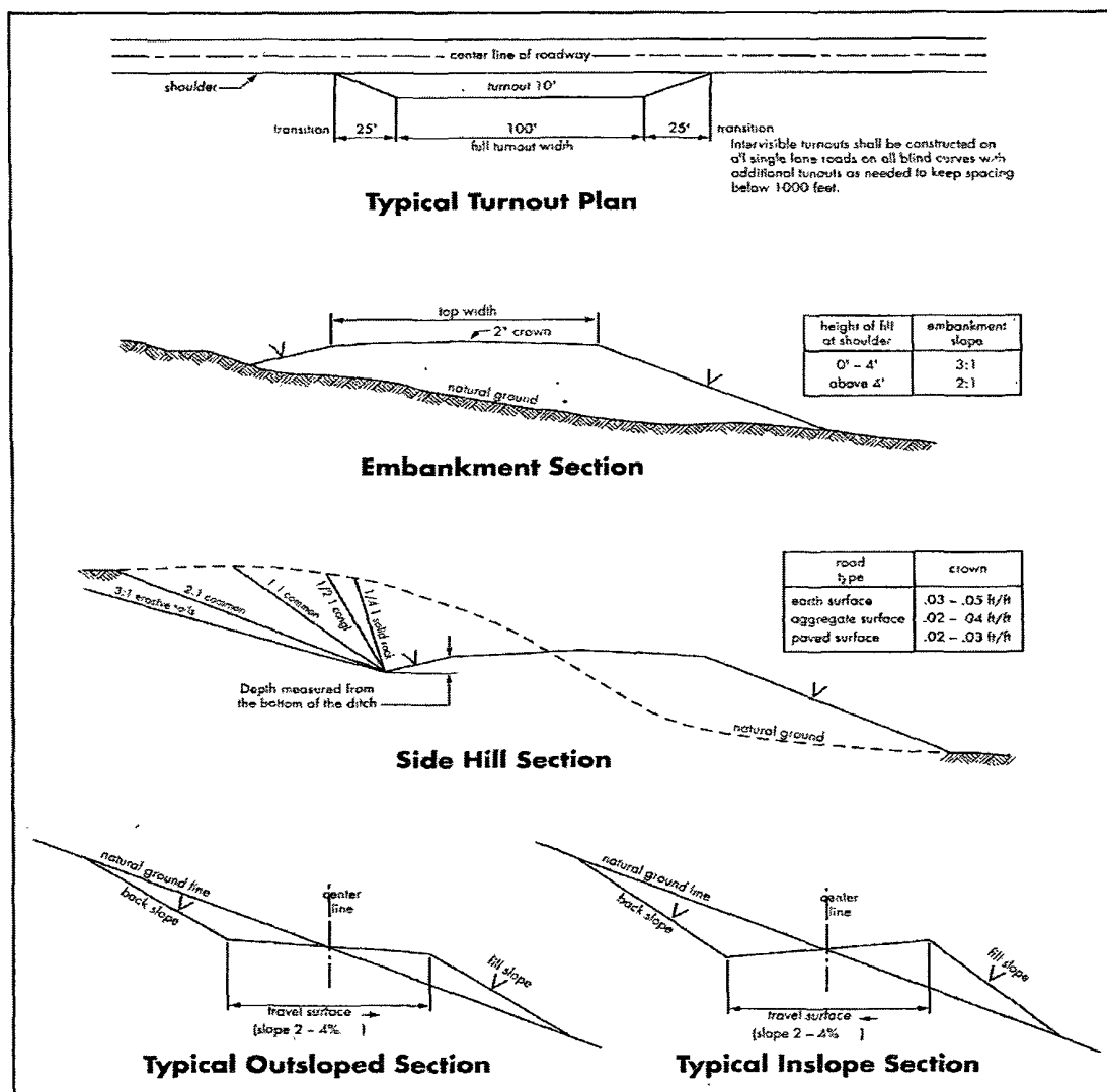
Figure 1 – Cross Sections and Plans For Typical Road Sections
