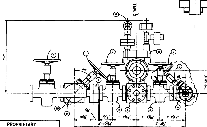
ELEVATION VIEW
