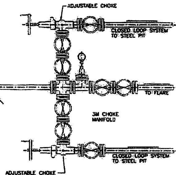
CHOKE MANIFOLD PLAN
