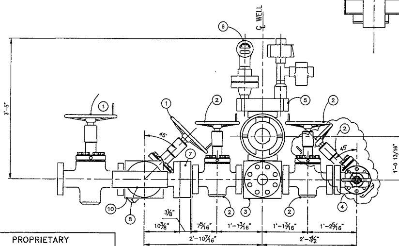
ELEVATION VIEW
