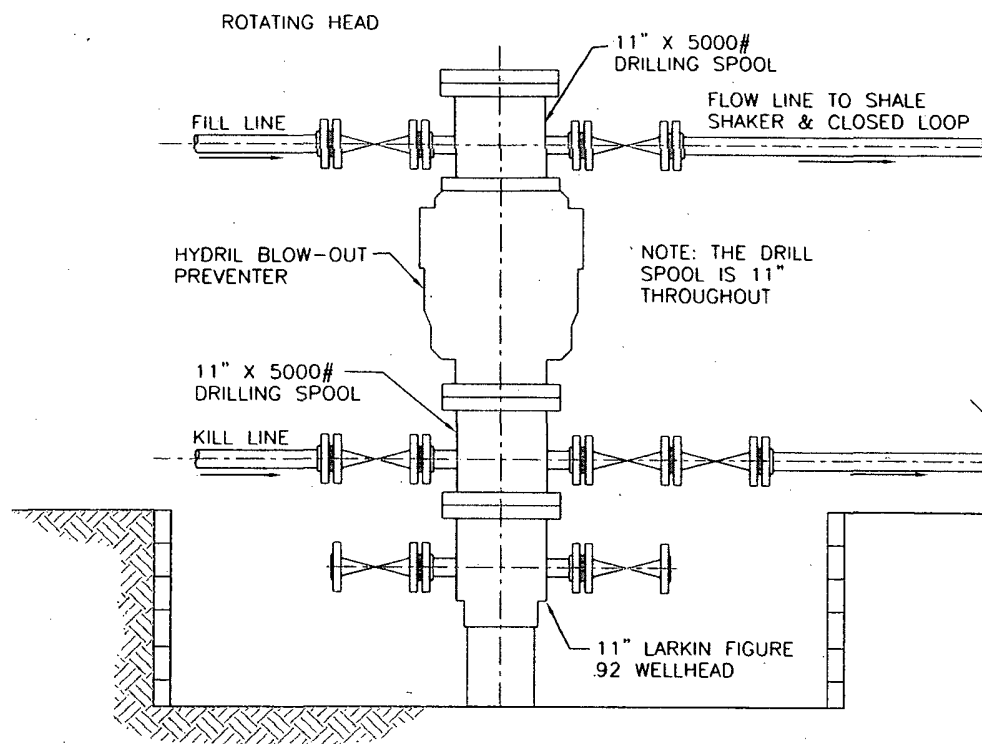
WELLHEAD ELEVATION
