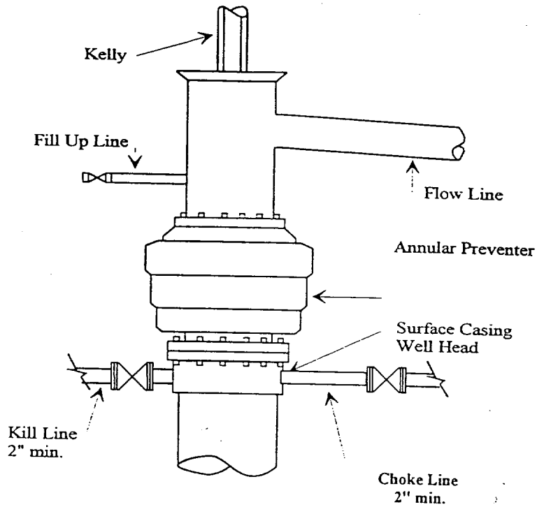
Typical 2,000 psi choke manifold assembly with at least these minimum features
