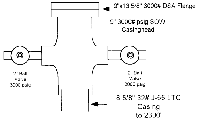
Wellhead Equipment Production Profile: 2300'-TD
