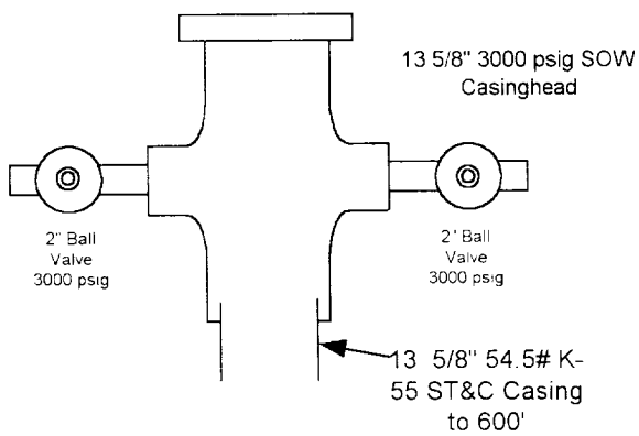
Wellhead Equipment Protective Profile: 600'-2300'
