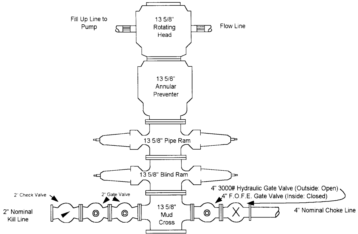
Wellhead Equipment Production Profile: 2300'-TD
