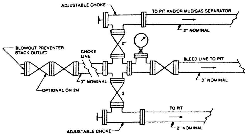
FIGURE K4-1. Typical choke manifold assembly for 2M and 3M ram working pressure service — surface installation.
