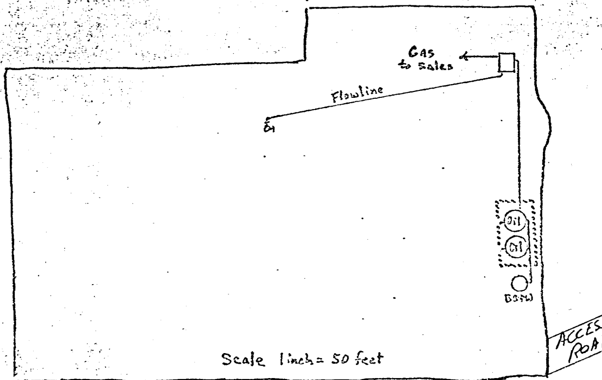
Tank Battery Layout
