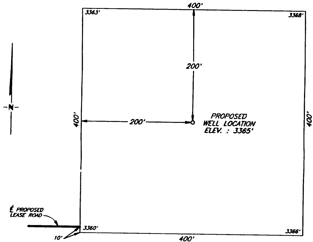
DETAIL VIEW 1" = 100'
