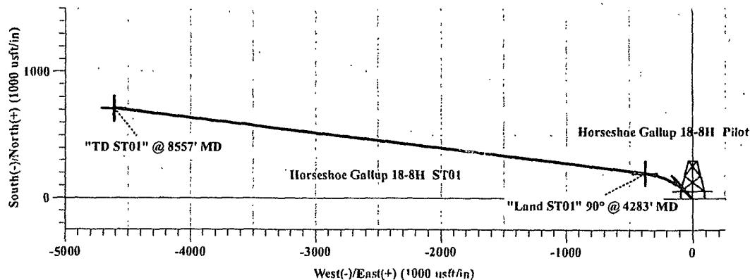
WELL DETAILS: Horseshoe Gallup 18-8H
