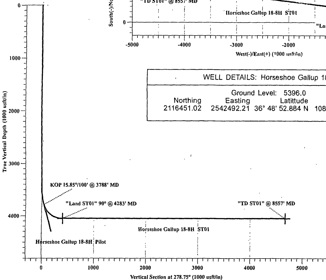
SECTION DETAILS
