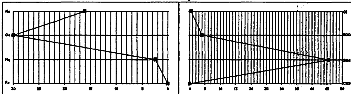
Stiff Diagram
