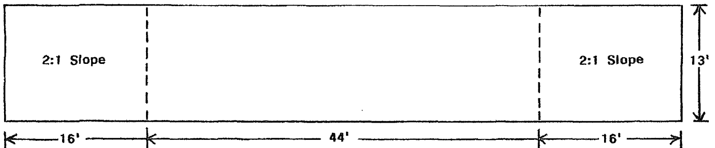
PLAN VIEW
