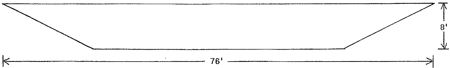
CROSS-SECTION LENGTH
