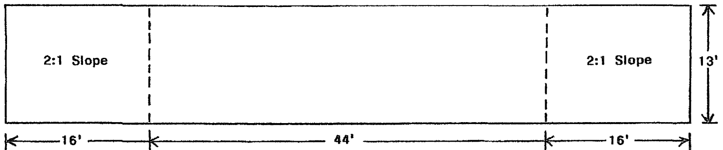
PLAN VIEW
