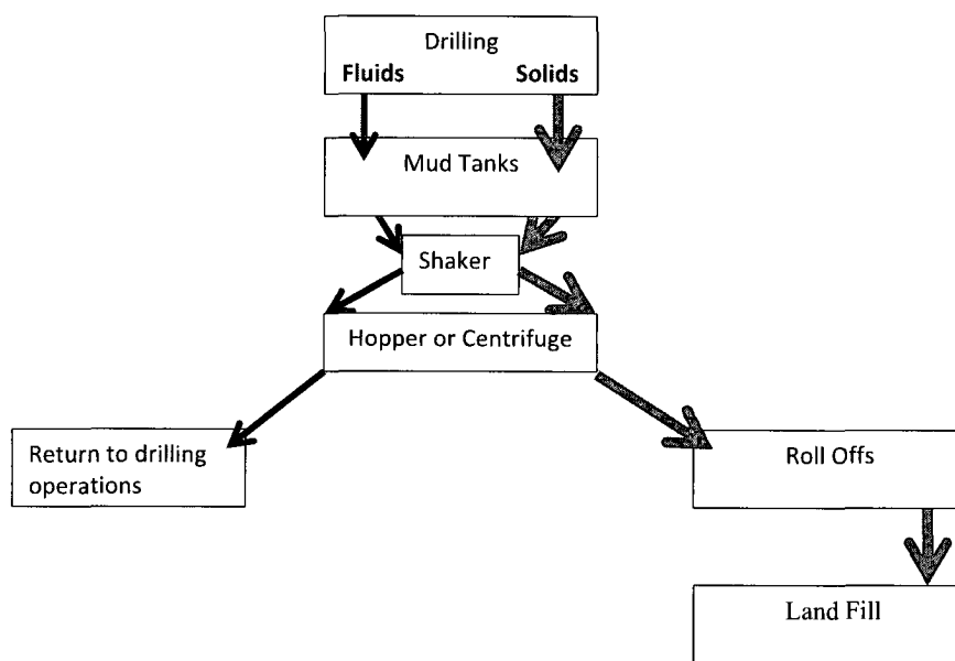
Flow Chart for Drilling Fluids and Solids
