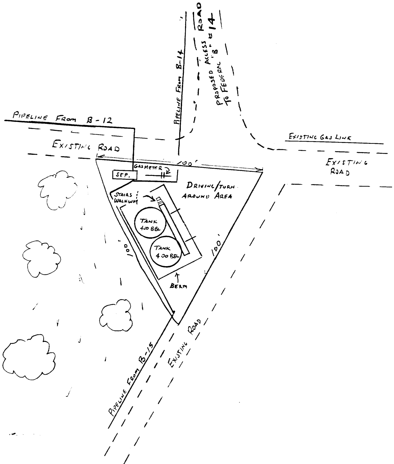
Exhibit "J" Central Facility Layout Federal "B" No. 12, 14, & 15 2400' FSL x 650' FEL Sec 27 T23N R7W Sandoval County, NM
