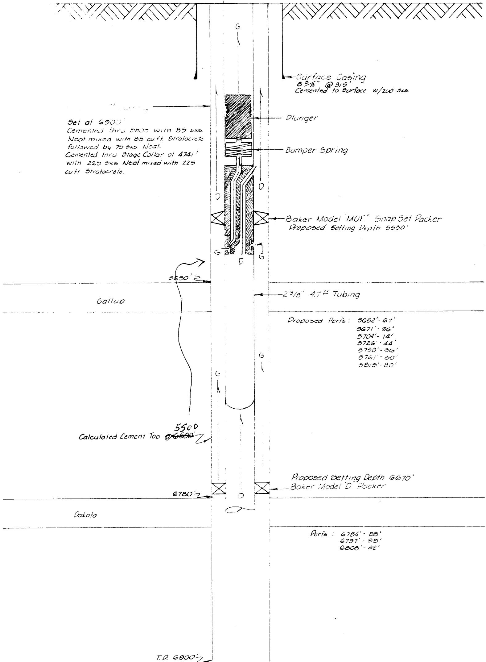
SCHEMATIC DIAGRAM of DUAL COMPLETION of NE HAYNES WELL 8 CONTINENTAL OIL CO. Dakota & Gallup Formations.
